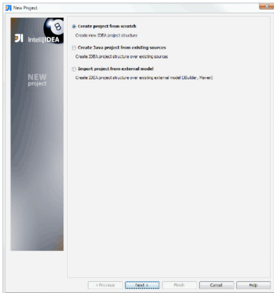
Figure 2-1. Starting IntelliJ
