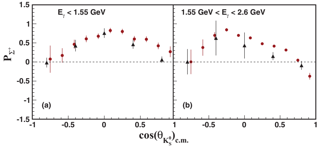
FIG. 8. (Color online) Comparison of polarization of \Sigma^+ between this result (circle) and SAPHIR (triangle) [17] for two different photon energy ranges. The photon energy range in (a) is from threshold to 1.55 GeV.
