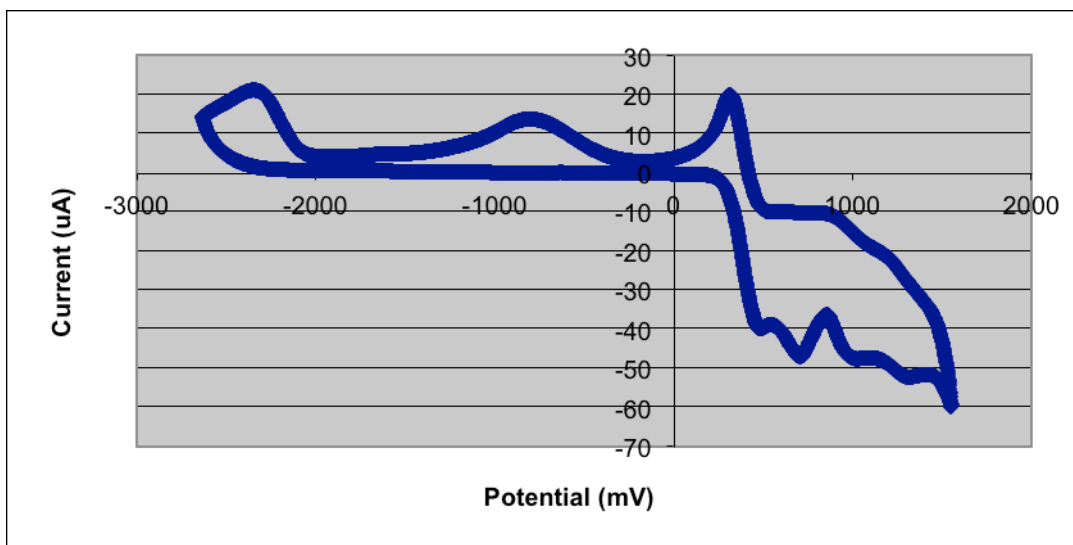
Fig. 8. Cyclic Voltammogram of 8 in DMSO (5.6 mM) with 0.2 M TBAF. The scan rate was 100 mV/s with ferrocene ( E_{1/2} = 400 mV) used as an internal standard.
