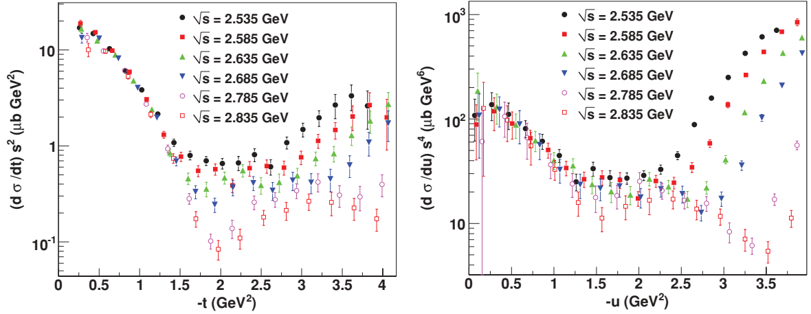
FIG. 16. (Color online) Regge scaling at high s for (a) t -channel (forward-angle) and (b) u -channel (backward-angle) nonresonant processes. The different marker colors and symbols correspond to different \sqrt{s} . The scaling behavior appears as the convergent set of points as t \rightarrow 0 or u \rightarrow 0 .
