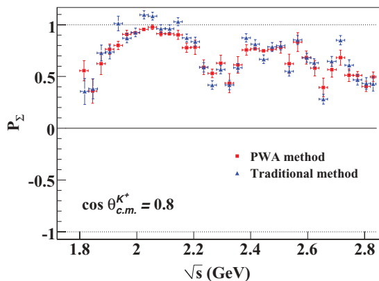
FIG. 12. (Color online) Comparison of the three-track P_{\Sigma} obtained from the partial-wave-expansion approach of Eq. (16) (red squares) and the more traditional intensity fit based approach of Eq. (19) (blue triangles). The agreement is excellent. At places where P_{\Sigma} approaches unity, the intensity method polarizations tend to overshoot slightly. The uncertainties for the PWA method are calculated indirectly from the statistical spread in the data, while the traditional method uncertainties directly come from the covariance matrix of a fit.
