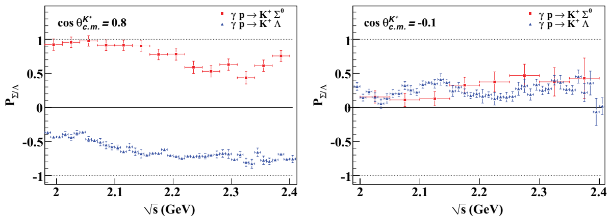
FIG. 17. (Color online) The SU(6) prediction of P_\Sigma \approx -P_\Lambda is seen to hold at (a) forward angles, but is broken for certain (b) mid- and backward-angle kinematics. The P_\Lambda values are taken from Ref. [25].
