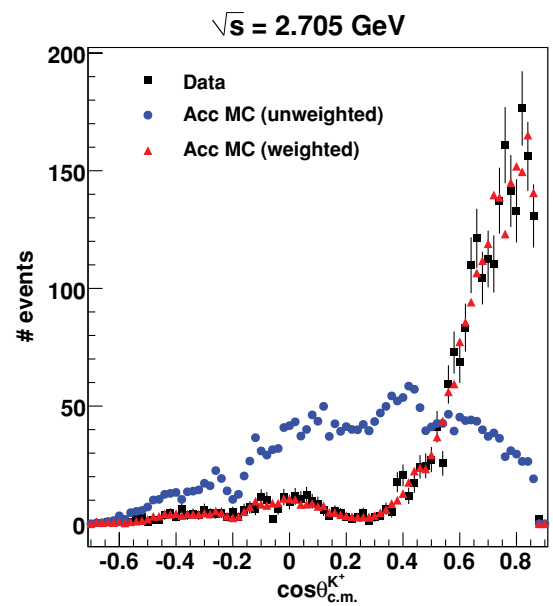
FIG. 6. (Color online) Shown are the \cos \theta_{c.m.}^{K^+} distributions for the data, accepted Monte Carlo and accepted Monte Carlo weighted by the PWA fit in the \sqrt{s} = 2.705 GeV bin for the three-track data set. Weighting by the fit results brings the weighted Monte Carlo distribution into excellent agreement with the real data.
