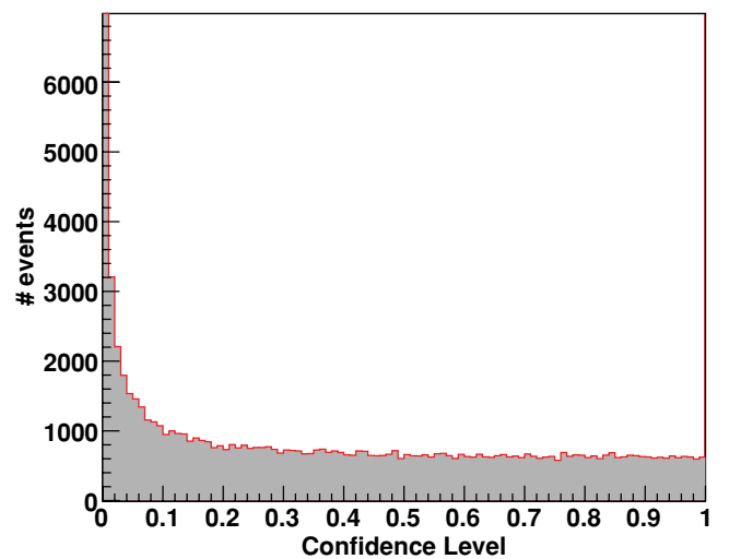
FIG. 1. (Color online) Confidence levels from a kinematic fit to the \gamma p \rightarrow K^+p\pi^-(\gamma) reaction topology. The distribution was fairly flat above \sim 10\% , as expected for real signal events. Background events mostly occupied the region about zero. These were removed by placing a loose 1% cut on the confidence level.
