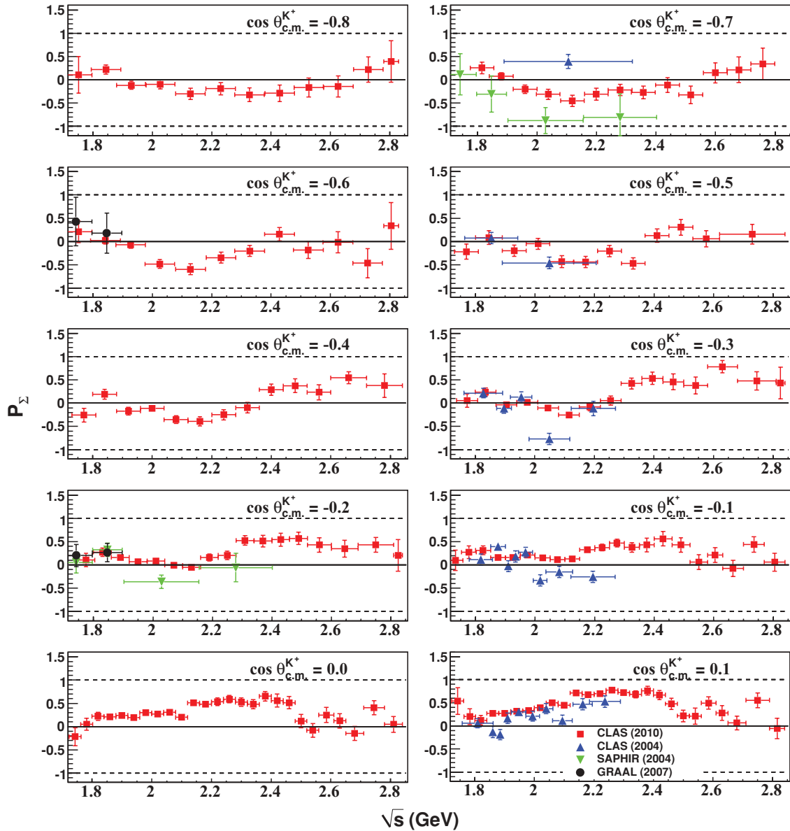
FIG. 13. (Color online) P_{\Sigma} vs. \sqrt{s} : Recoil polarization world data in the backward angles. CLAS (present analysis) results are in red squares, earlier CLAS [13] results in blue up-triangles, SAPHIR [16] in green down-triangles, GRAAL [19] are in black circles. The error bars represent the statistical uncertainties.
