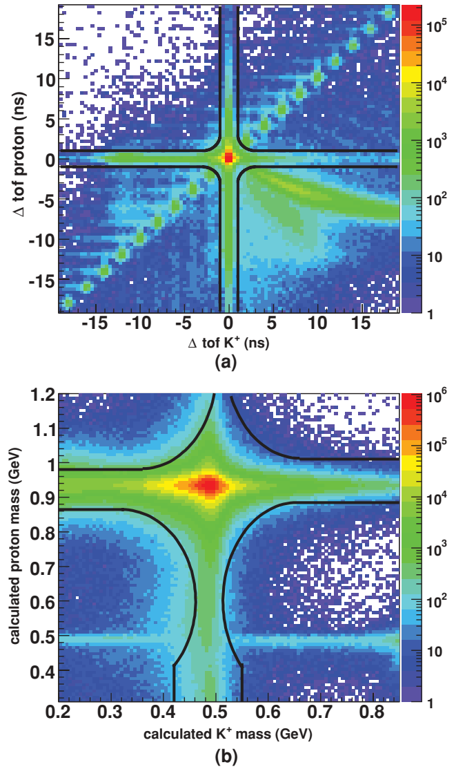
FIG. 2. (Color online) Timing cuts for background removal: (a) three-track topology and (b) two-track topology. Events lying outside the quadrant of black curves in both figures were removed from further analysis. Note the logarithmic scale for the intensity axes.
