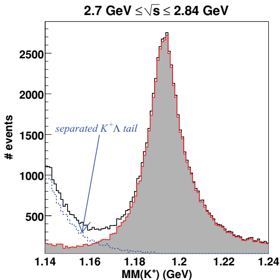
FIG. 3. (Color online) Effect of the K^+\Lambda removal cut: for the three-track topology, instead of fitting to \gamma p \rightarrow K^+ p \pi^-(\gamma) for K^+\Sigma^0 events, we can fit to \gamma p \rightarrow K^+ p \pi^- (nothing missing) for K^+\Lambda . By rejecting events with confidence level >0.1\% for the latter hypothesis, we can remove the K^+\Lambda background tail effectively (dotted histogram in blue). Only events in the shaded histogram were kept after this cut.
