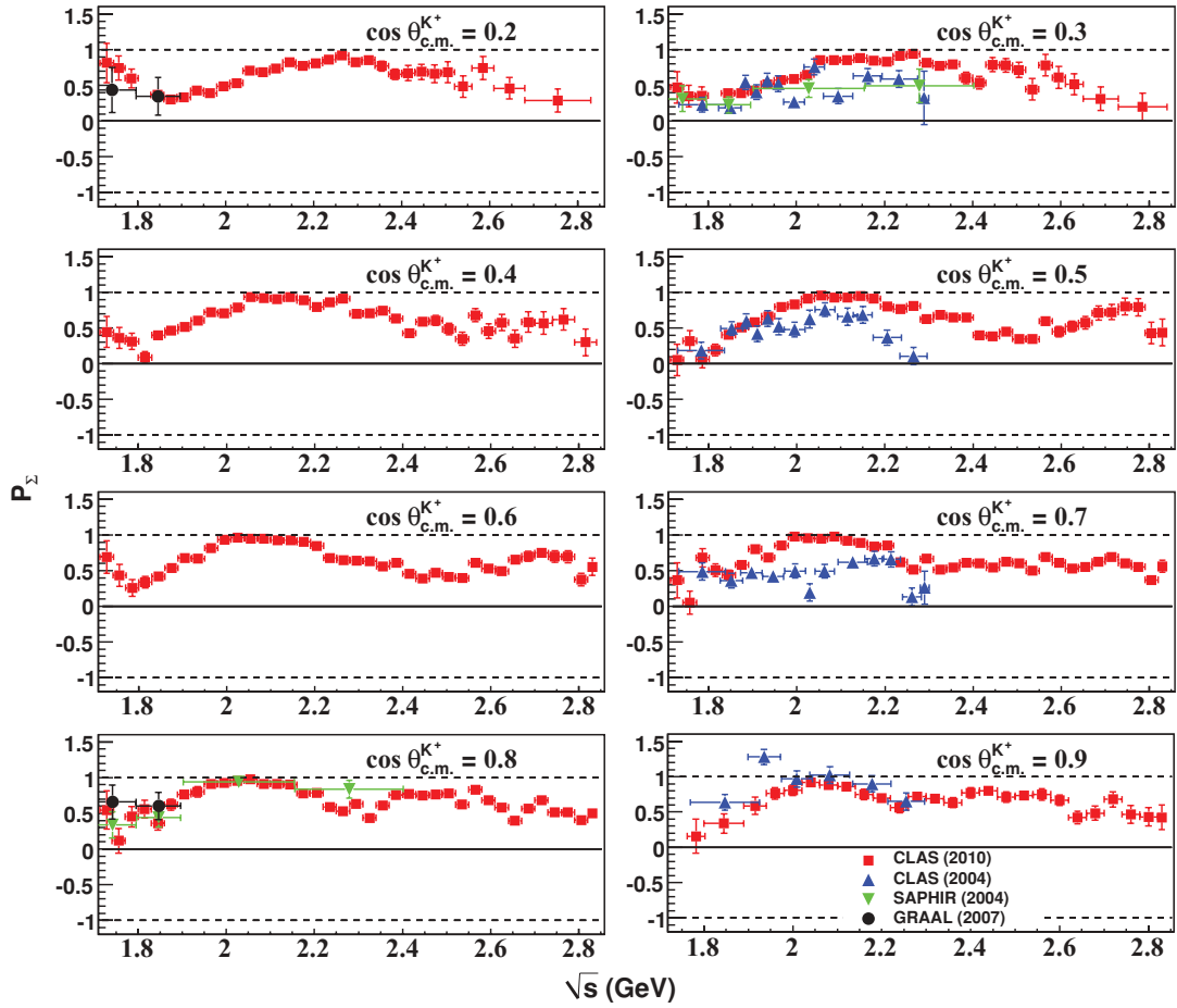
FIG. 14. (Color online) P_\Sigma vs. \sqrt{s} : Recoil polarization world data in the forward angles. CLAS (present analysis) results are in red squares, earlier CLAS [13] results in blue up-triangles, SAPHIR [16] in green down-triangles, GRAAL [19] are in black circles. The error bars represent the statistical uncertainties.
