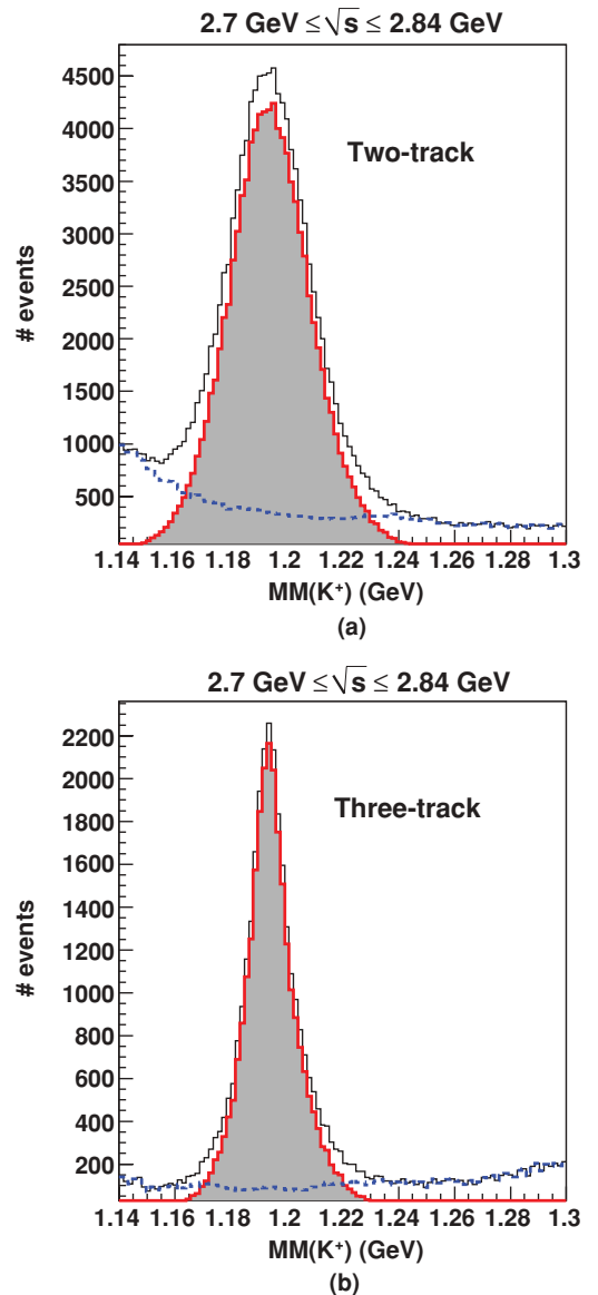
FIG. 5. (Color online) Signal-background separation in the high \sqrt{s} regions integrated over all angles for (a) two-track and (b) three-track topologies. The red (shaded) histograms are the data weighted by Q , representing the signal, while the blue (dotted) histograms are the data weighted by (1 - Q) , representing the background. Note that the three-track data set has a smaller background from the K^+\Lambda “tail” because of the additional cut described in subsection IV B.
