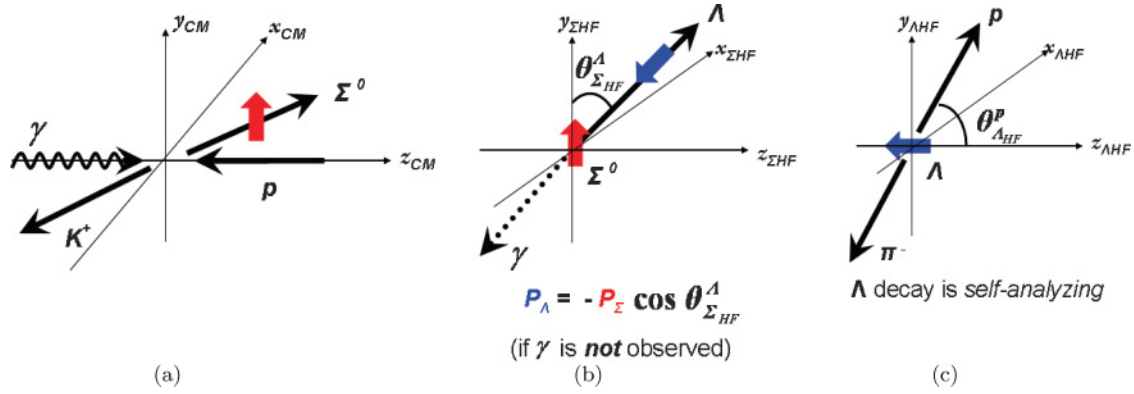
FIG. 7. (Color online) A pictorial representation of the helicity angles \theta_{\Sigma_{\text{HF}}}^{\Lambda} and \theta_{\Lambda_{\text{HF}}}^p and the polarization transfer between the \Sigma^0 and the \Lambda . (a) Shows the \gamma p \rightarrow K^+ \Sigma^0 reaction in the center-of-mass frame with the y axis as the normal to the production plane. The only component of the induced \Sigma^0 spin measurable in the current experiment is along the normal to the production plane, shown by the bold arrow in red. (b) Shows the \Sigma^0 \rightarrow \Lambda \gamma decay in the \Sigma^0 helicity frame and (c) shows the \Lambda \rightarrow p \pi^- decay in the \Lambda helicity frame. See text for details.
