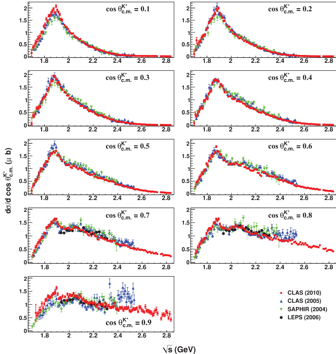
FIG. 11. (Color online) \frac{d\sigma}{d\cos\theta_{c.m.}^{K^+}} ( \mu\text{b} ) vs. \sqrt{s} in the forward angles: final CLAS (present analysis) differential-cross-section results as the weighted average of the two topologies are in red squares. Previous CLAS results [14] are in blue up-triangles while green down-triangles are results from SAPHIR [16]. The black circles represent LEPS measurements [17] in the forward-most angular bins. All error bars represent statistical uncertainties only.
