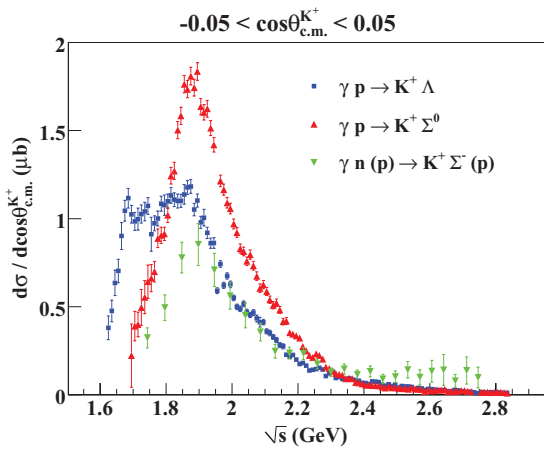
FIG. 15. (Color online) Differential cross sections at \theta_{c.m.}^{K^+} = 90^\circ for \Lambda [25] (blue squares) and \Sigma^0 (red up-triangles) photoproduction from proton and \Sigma^- [39] (green down-triangles) photoproduction from deuteron. Except for the extreme forward angles, all three hyperon channels show a similar peak at \sqrt{s} \sim 1.9 GeV.
