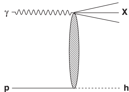
FIG. 22. Schematic representation of the leading-particle target fragmentation mechanism. The hatched blob represents the structure function of a particle or a set of particles exchanged. In case of \pi^+ production the first particle in the blob is the neutron.
