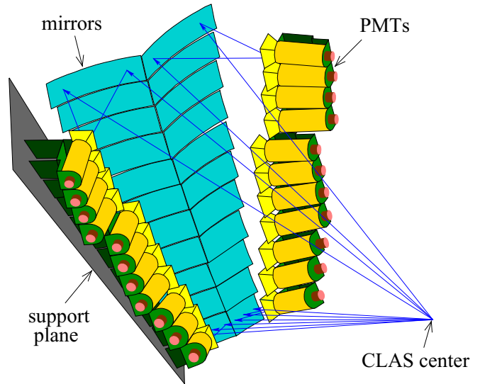
FIG. 3. The new Cerenkov detector designed and built by the INFN-Genova group. It consists of 11 pairs of mirrors with spherical curvature, which reflect the Cherenkov light to corresponding photomultiplier tubes (PMTs). Only one of the two support planes for the PMTs is shown here. The solid blue lines show simulated particle trajectories originated from the CLAS center and the reflection of the Cherenkov light towards the PMT.
