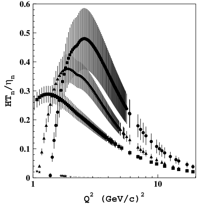
FIG. 13. Ratio of the total higher twist [see Eq. (24)] to the leading twist given in Eq. (21) with its systematic uncertainties. (Stars) M_2 ; (squares) M_4 ; (triangles) M_6 ; (circles) M_8 .
